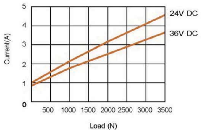
Current vs Load
