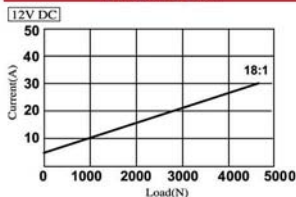
Current vs Load
