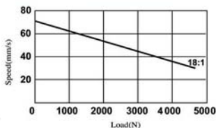
Speed vs Load
