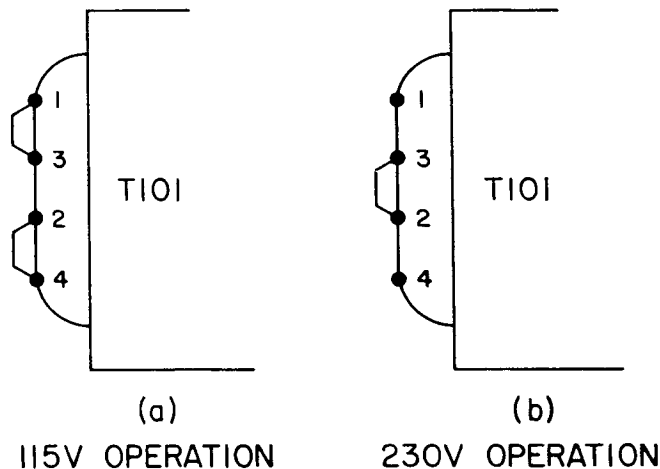
Figure 9. AC Input Wiring Diagram
