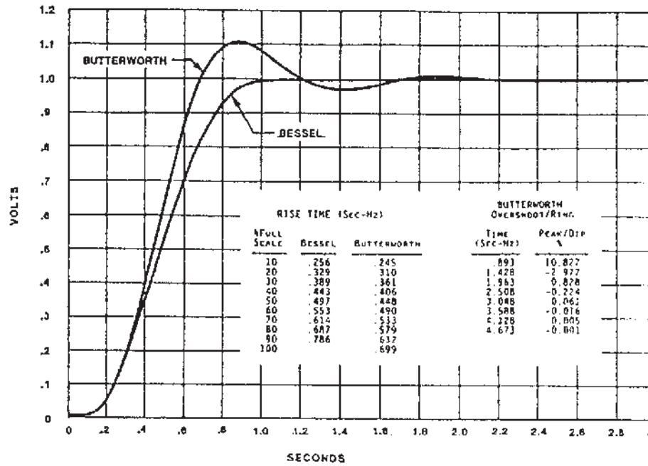
Figure 2.4 Transient Response
