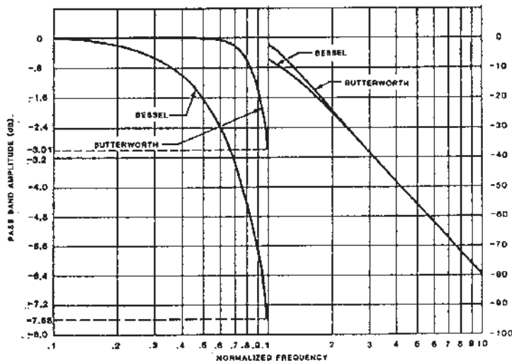
Figure 2.1B Low-Pass Amplitude Response
