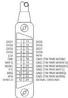
Figure 3.1 Rear Panel GPIB Connector
