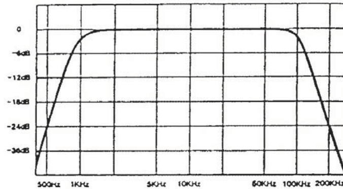
Figure 4.1 Band-Pass Response
