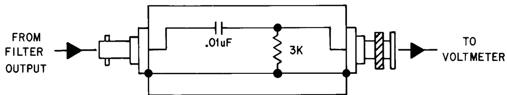
Figure 4.3 High-Pass Filter
