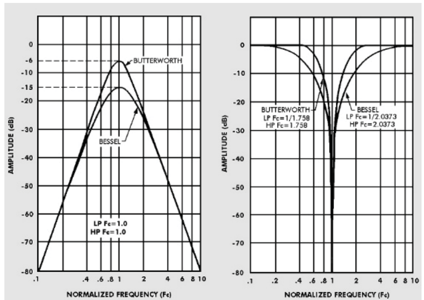
Figure 4.1 Band-Pass Response
