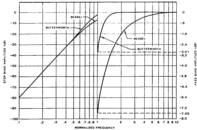
Figure 2.5 High-Pass Response
