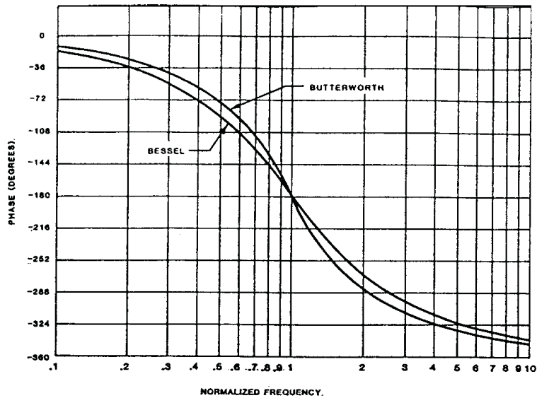
Figure 2.6 Low-Pass Phase Response
