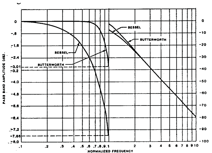
Figure 2.4 Low-Pas Response
