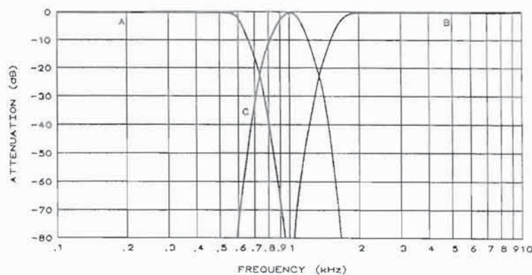
Figure 2.2 Band-Pass/Band-Reject Response
